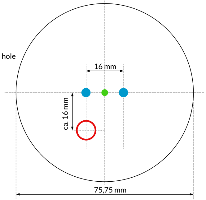
Drilling Template iSHearo
